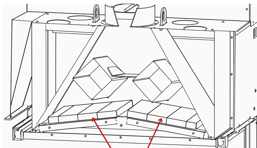
Baffle plates in position
